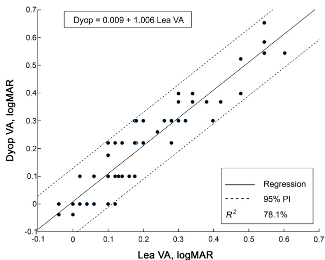
FIG 5. Linear regression of the Dyop visual acuity test against Lea numbers chart showing a strong linear correlation of 0.88 . The regression equation is Dyop visual acuity test = 0.009 + 1.006 (Lea numbers chart). PI , prediction interval.
